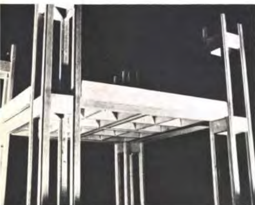
Fig. 21 Birmingham University, Mining & Metallurgy Building 1964. Study model of repetitive coffered element. Four columns 25 ft. bays
