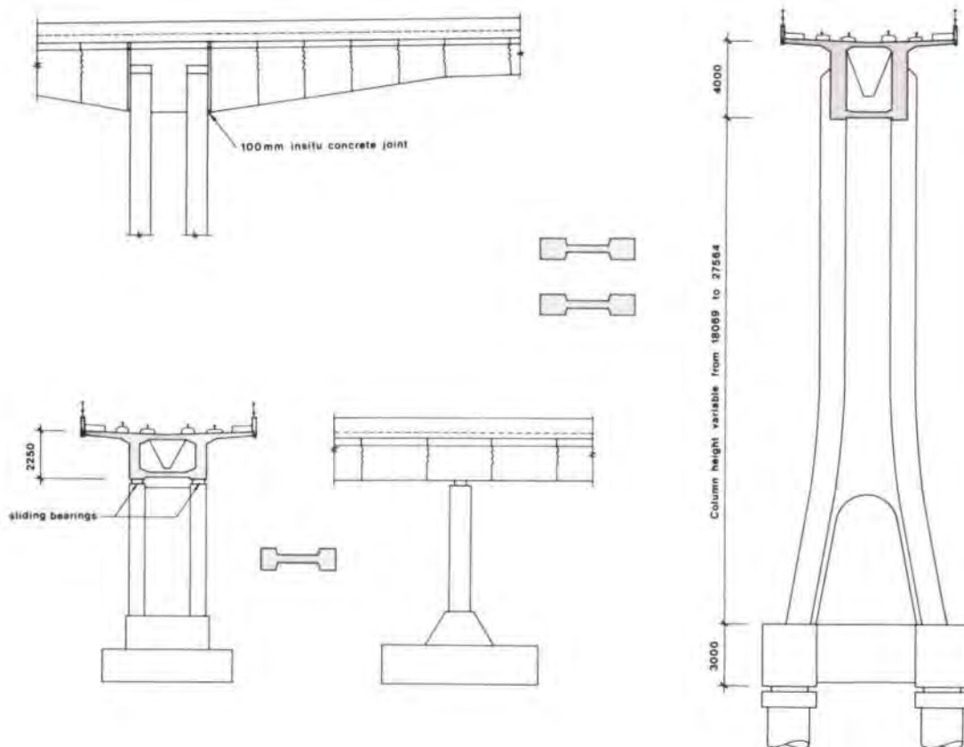
Fig. 7 Typical single column and typical double column
