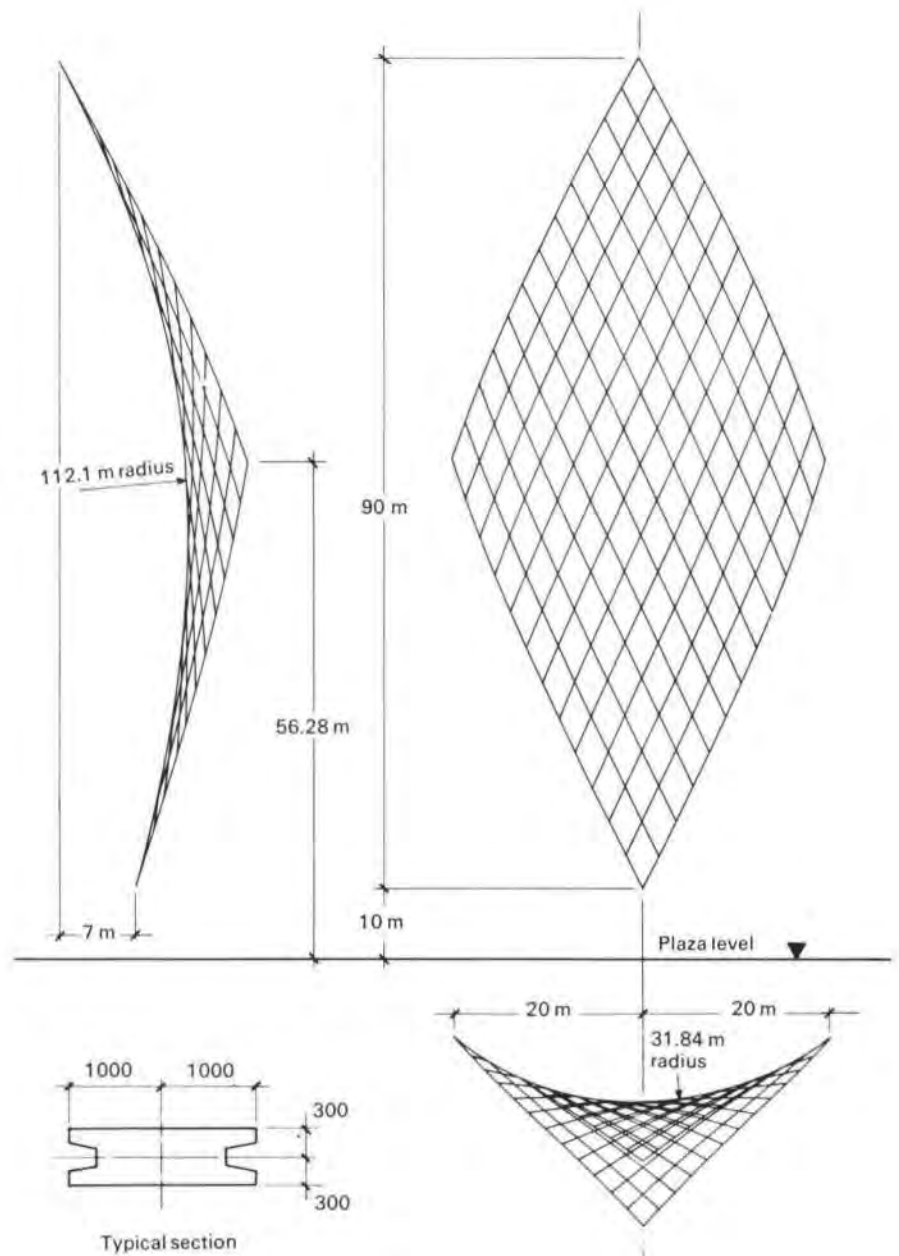
Fig. 6 Geometry
