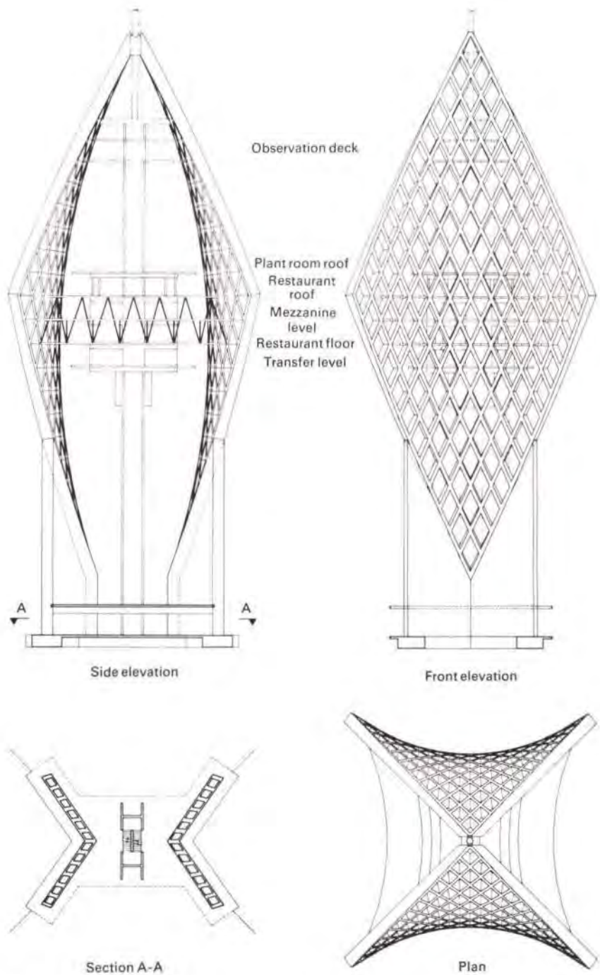
Fig. 3 Plan and elevations
