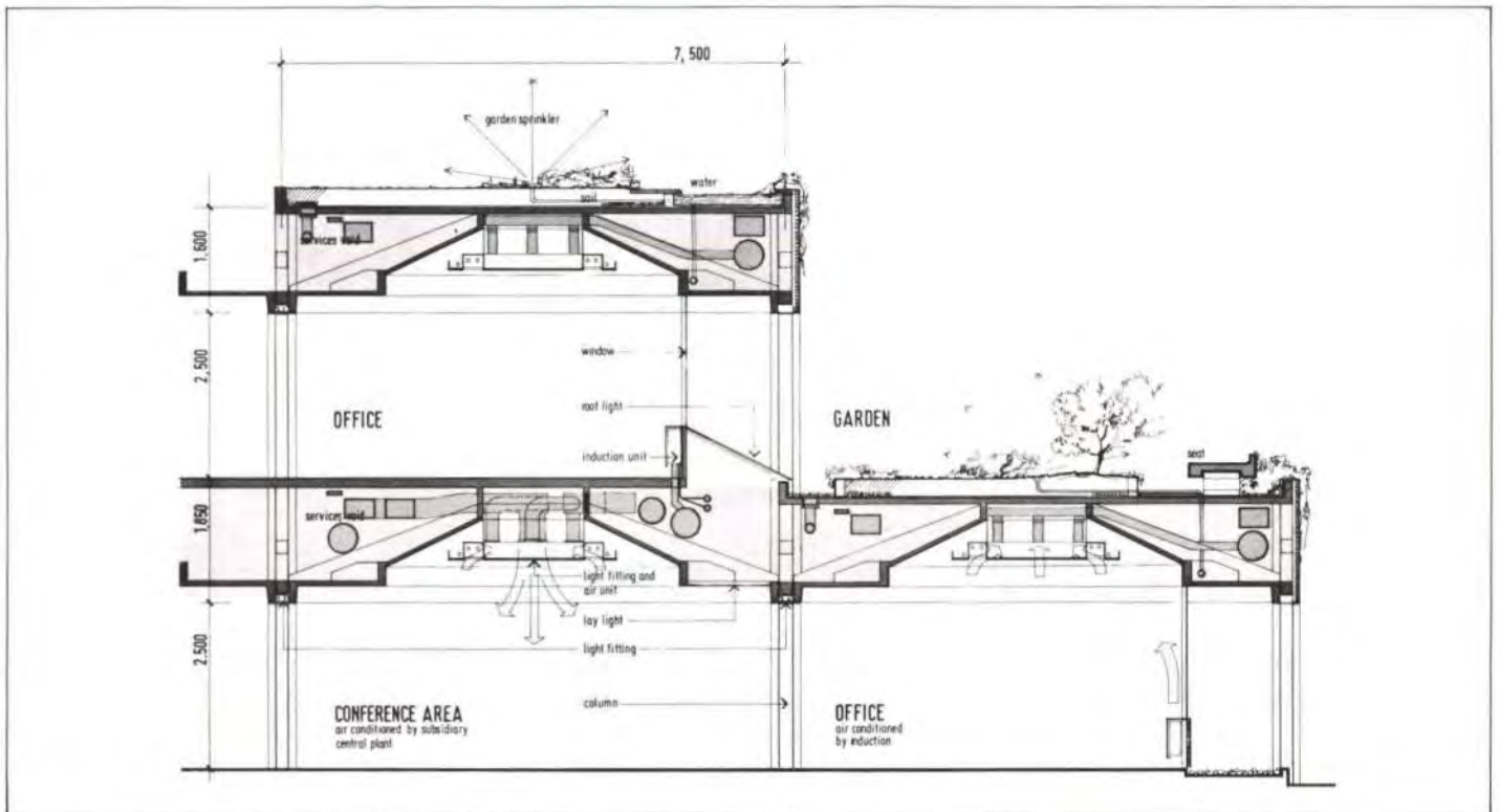
Fig. 18 below Wiggins Teape: section showing repeated pyramidal volumes. ‘Larger buildings require larger basic subdivisions’
