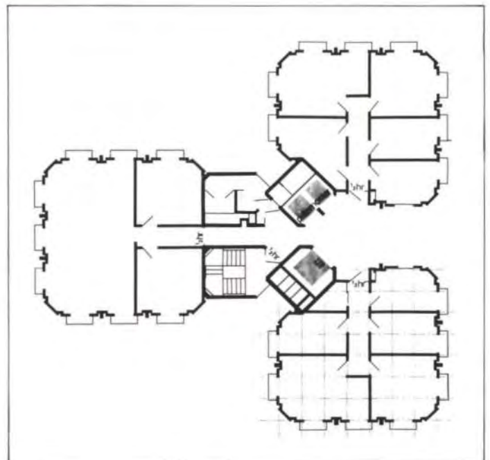
Fig. 55 Arts & Commerce tower: typical 'trefoil' floor plan. The whole building is naturally ventilated
