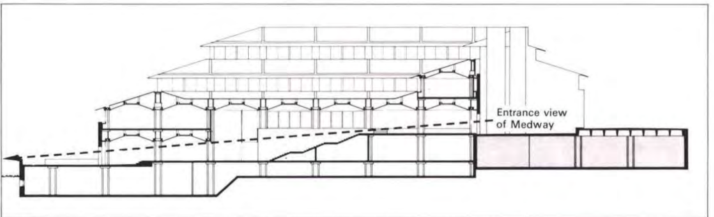
Fig. 12 Lloyd's: section showing relationship to site and primary circulation
