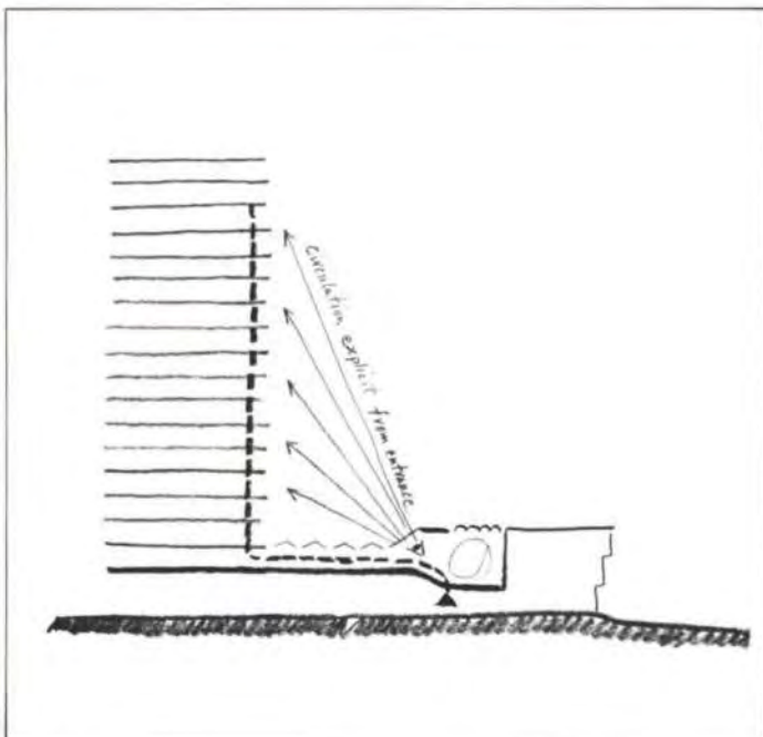
Fig. 54 Leicester Arts and Commerce tower: circulation diagram. Departmental colour coded lobby screens visible through glazed roof of entrance link. Destination thus signalled. Emphasis on an explicit circulation design
