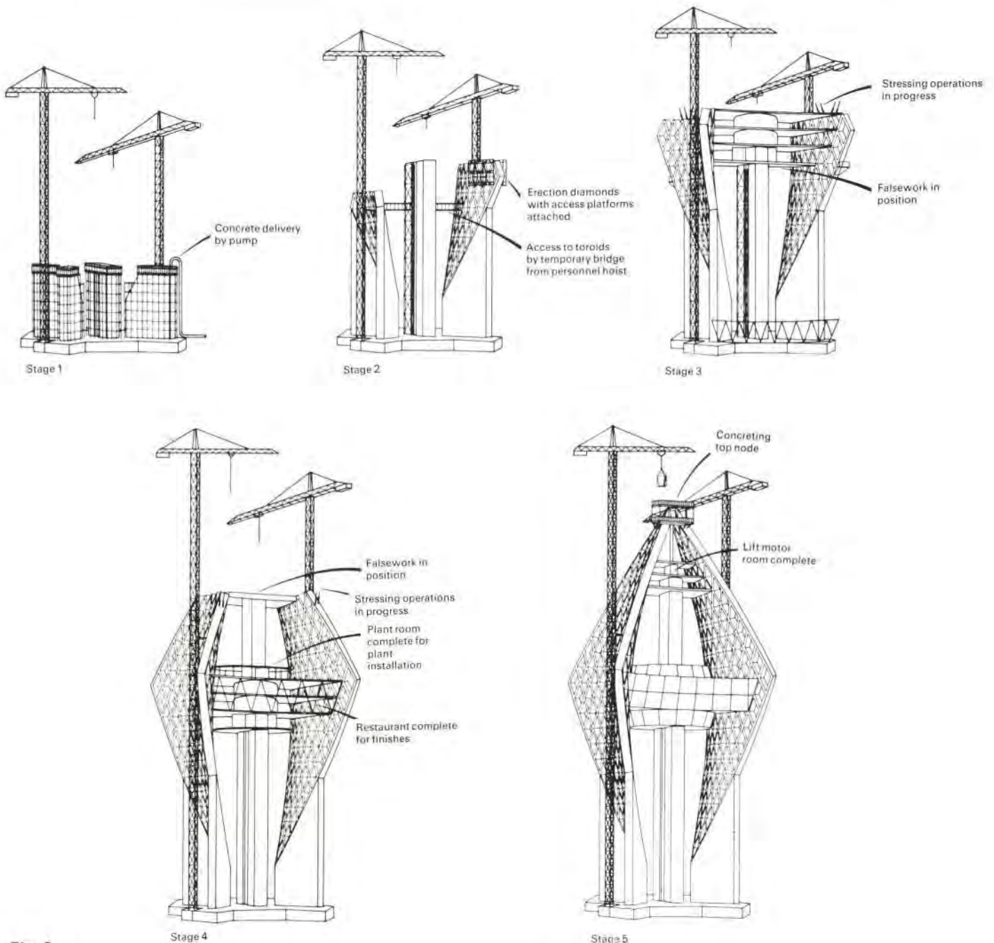
Fig. 8 Construction sequence
