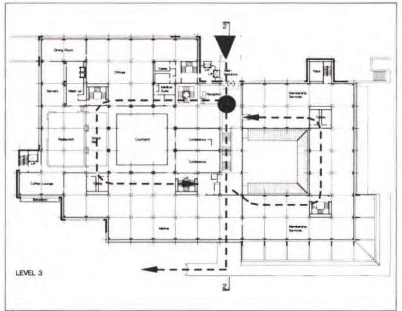
Fig. 11 Lloyd's Administrative Headquarters, Chatham: the planned circulation diagram
