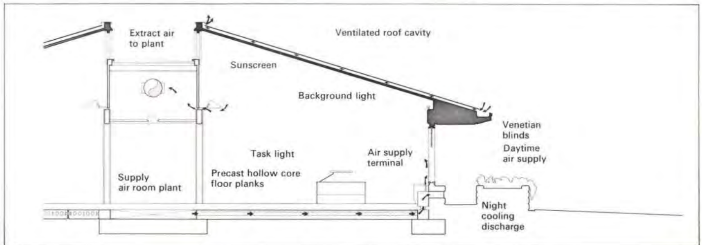
Fig. 43 CEGB cross-section: the thermal mass of the floor slabs cooled at night are used to modulate the internal environment by day
