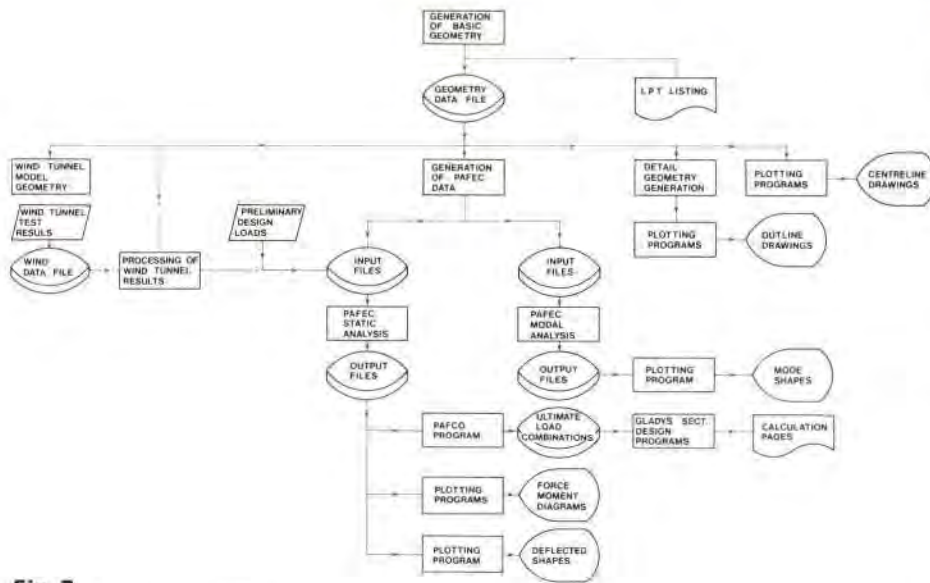
Fig. 7 Computer design flow chart
