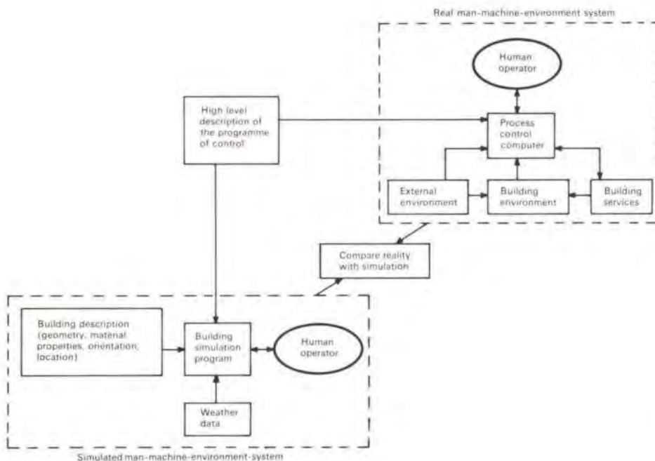
Fig. 4 If a human operator is included in the system then by designing the programme of control the building services designer is effectively designing the job of the human operator. The building simulation program can be run in 'real time' to simulate the control task for the human operator.
