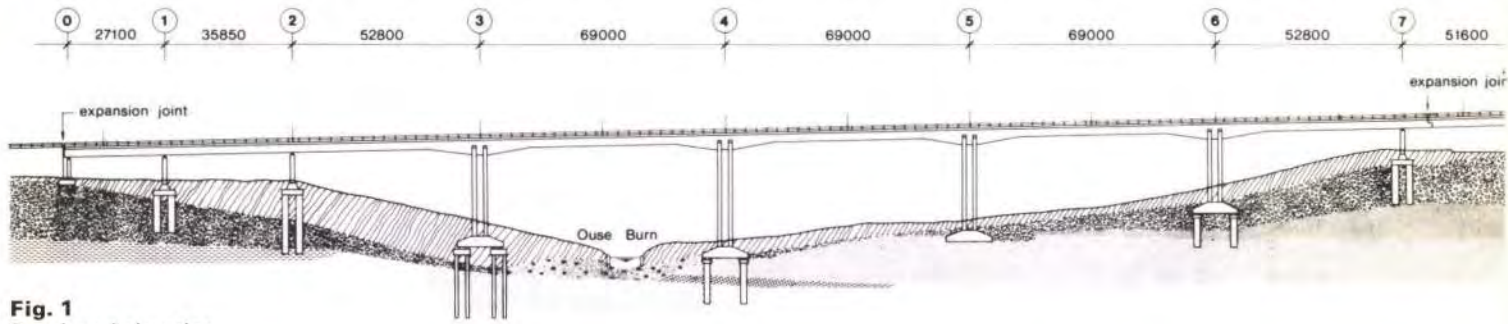
Fig. 1 Developed elevation
