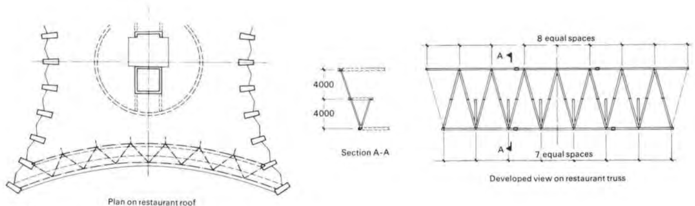
Fig. 4 Restaurant structure
