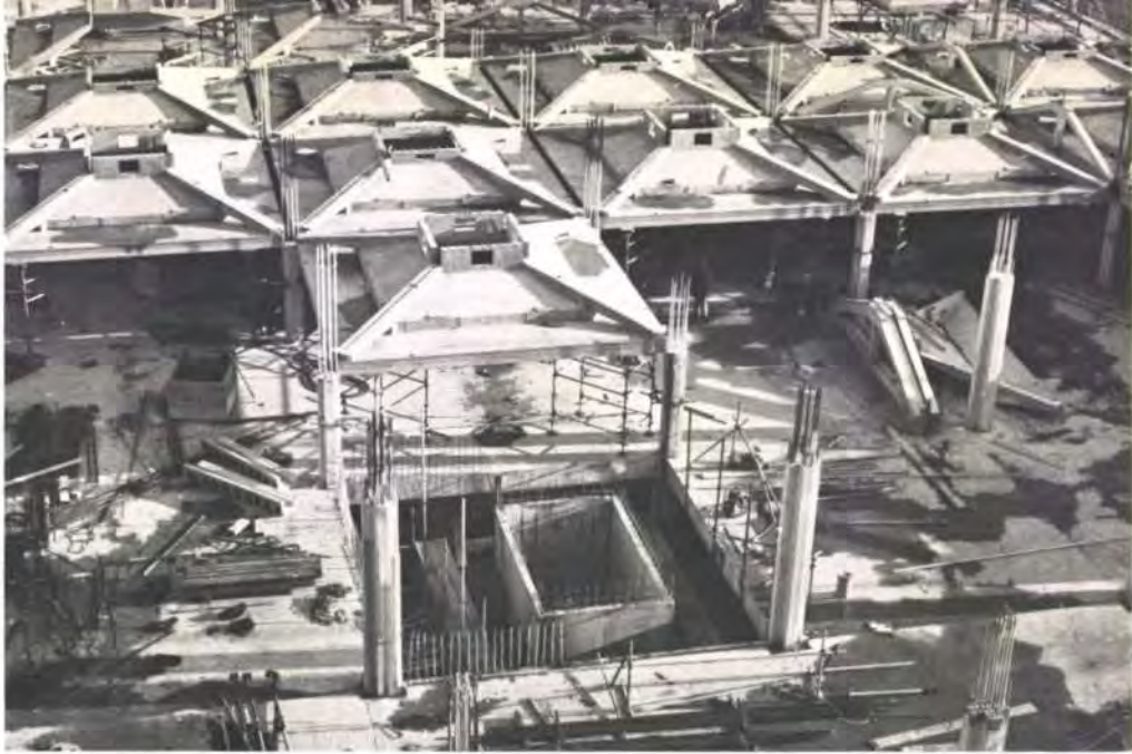
Fig. 19 Wiggins Teape under construction: 7.5 m bays with single columns and edge beams. Pyramids are precast in four pieces
