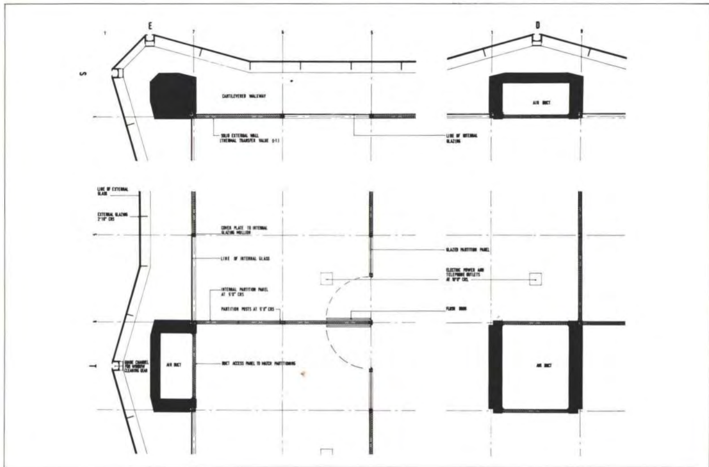
Fig. 48 IBM plan: typical corner with partition, grid and 'double skin'
