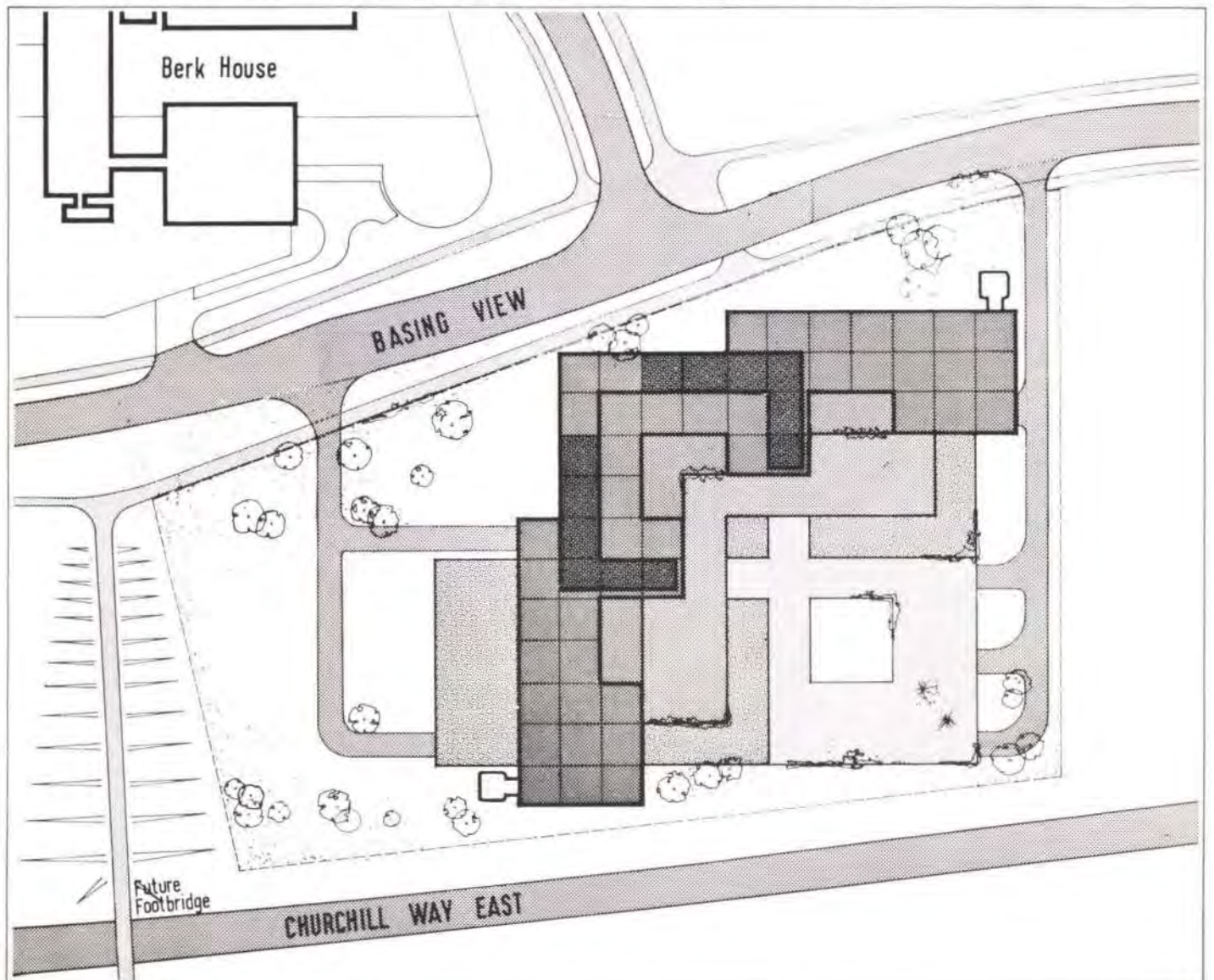
Fig. 31 Wiggins Teape: site plan: sloping site, stepped terraces
