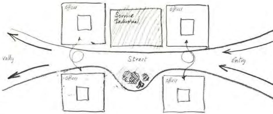
Fig. 7 left CEGB offices: plan diagram. From a central 'street' all the central communal activities, including banks, shops, staircases to restaurants, exhibition spaces, libraries and so on, are planned. The secondary groupings radiate from top-lit double height squares.
