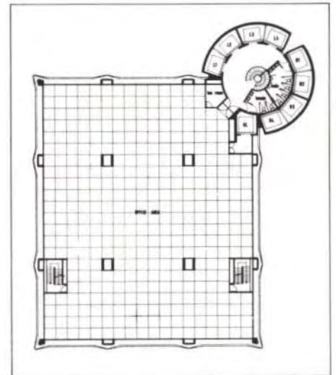
Fig. 46 IBM Johannesburg: typical plan
