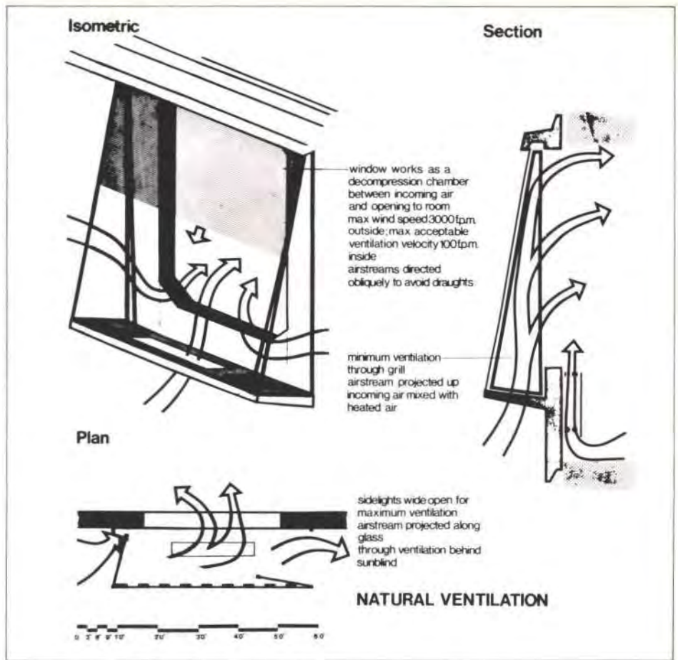
Fig. 39 Leicester University, Arts & Commerce Tower, 1964: diagram of the natural ventilation system
