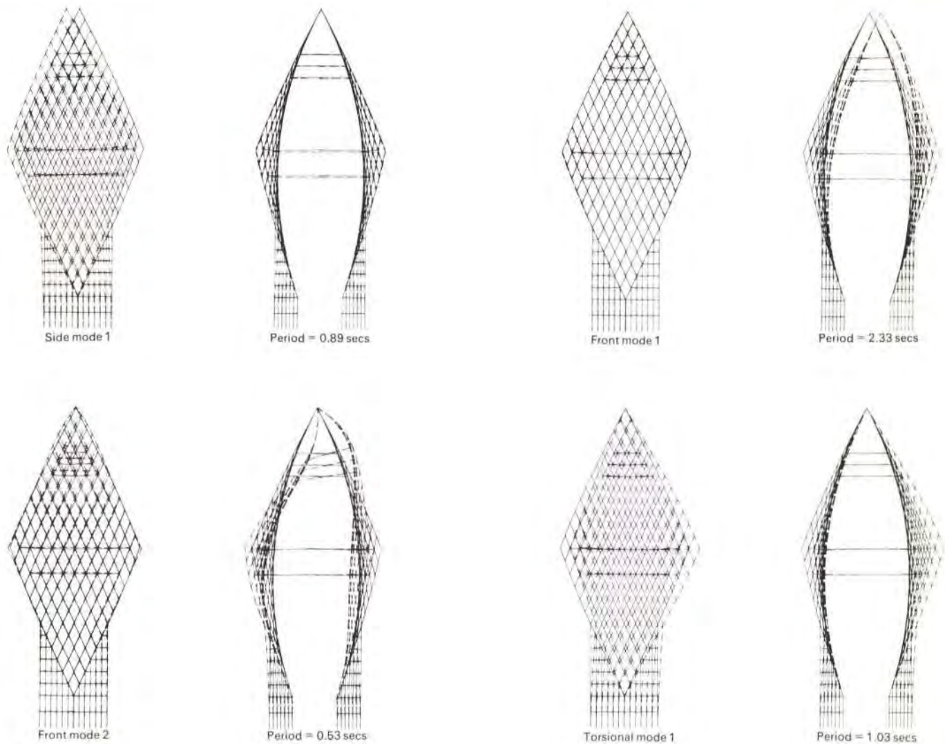
Fig. 9 Mode shapes
