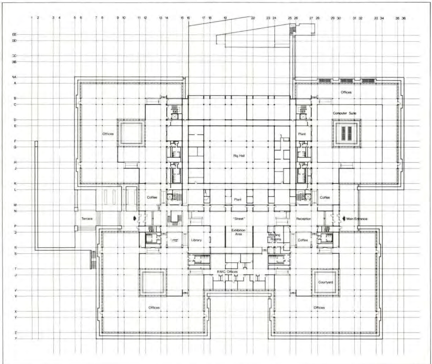
Fig. 8 below CEGB offices: plan at 'street' level
