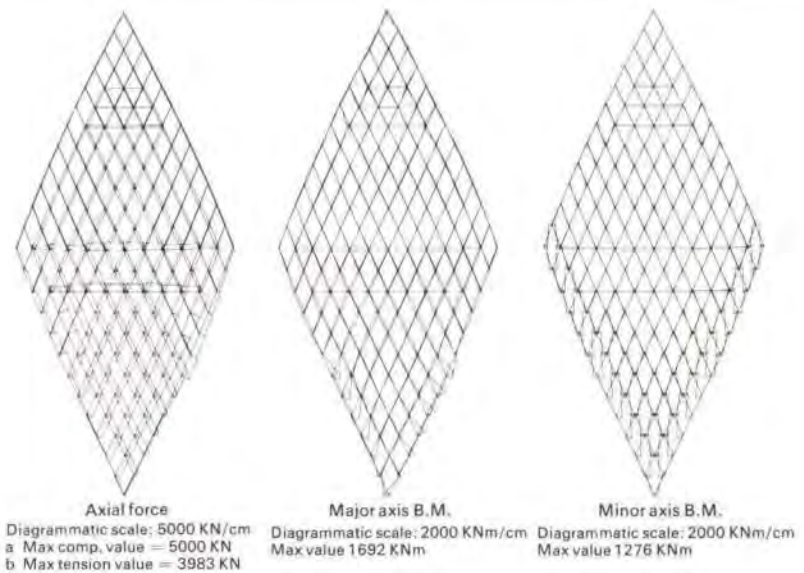
Fig. 5 Bending moment diagrams
