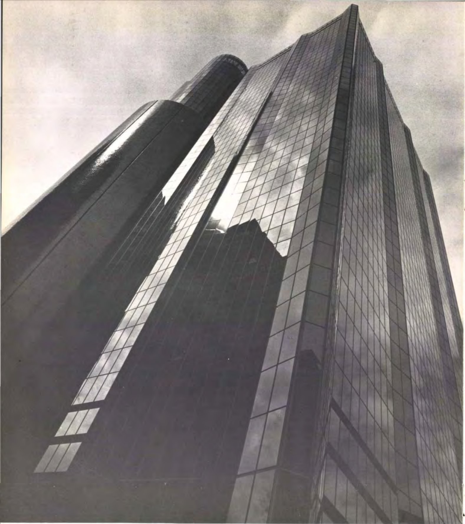
Fig. 49 IBM Johannesburg: circular service core with high and low rise lift shafts expressed
