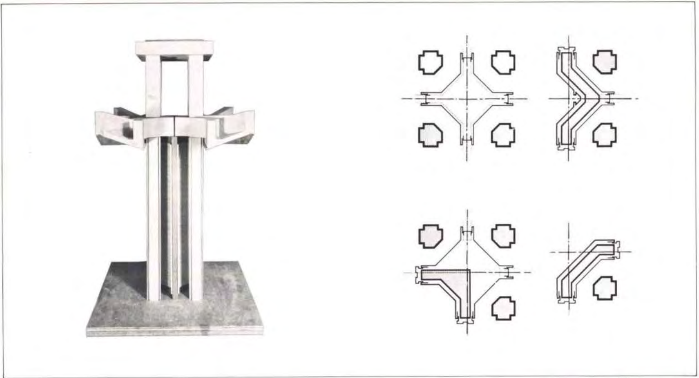
Fig. 26 Lloyd's: four column group with internal cruciform duct. Duct houses various services outlets and provides for partition fixing
