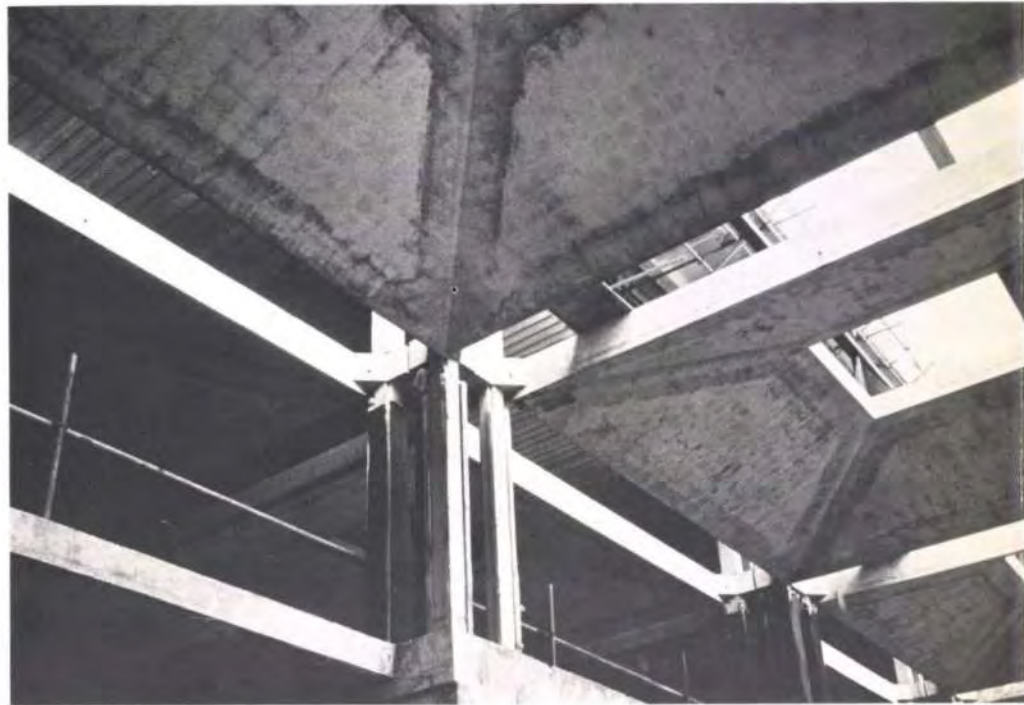
Fig. 26 Lloyd's: four column group with internal cruciform duct. Duct houses various services outlets and provides for partition fixing
