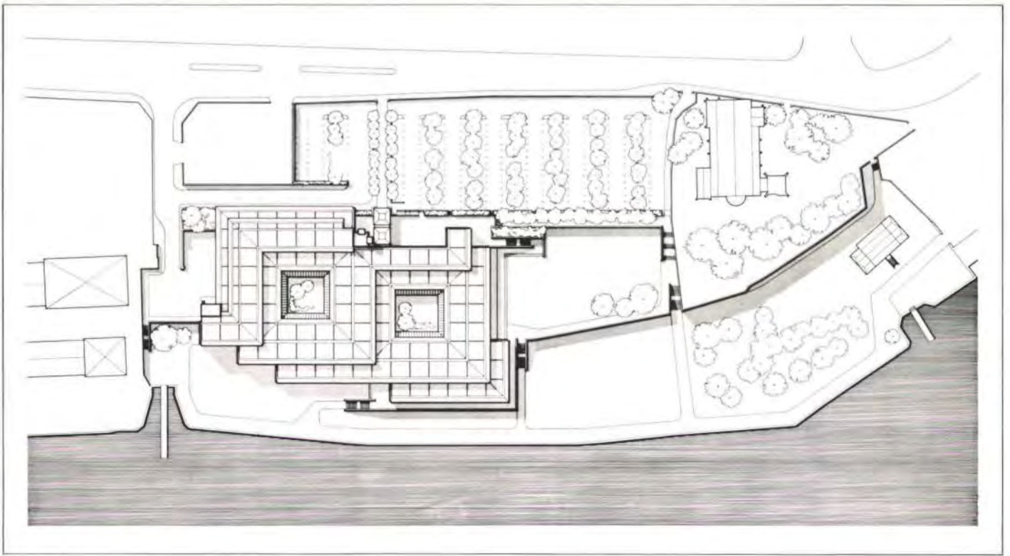
Fig. 9 Lloyd's, Chatham: site plan
