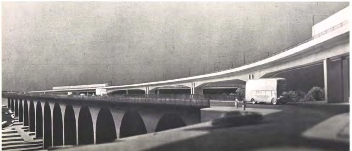
Fig. 3 The viaduct curves around to cross over the road. Pier number 7 is at right of picture
