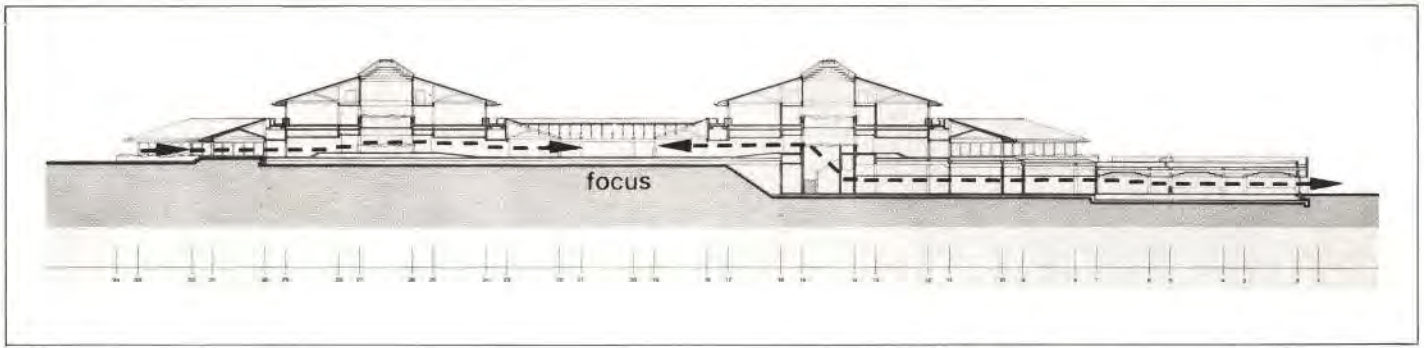
Fig. 6 above CEGB offices, Bedminster Down: section showing movement pattern
