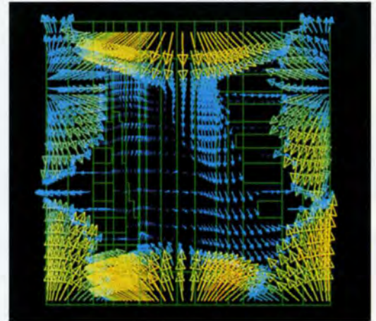
5. Air speed vectors during extreme summer condition.
