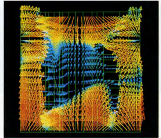
7. Air speed vectors during extreme winter condition.
