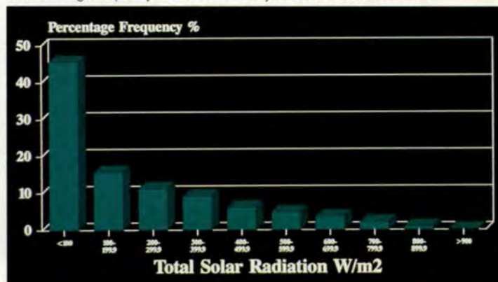
17. Percentage frequency distribution of hourly values of outdoor radiation.
