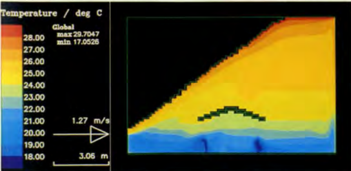
18. Summer airflow simulation hybrid system: natural ventilation and local spot cooling: ▲(a) air speed ▼(b) temperature
